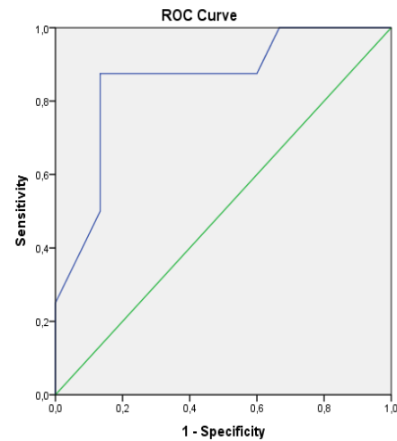
Figure 4. Receiver operating characteristic (ROC) analysis of increasing Beck depression scores and lower percentile (<33%) FORT ratios of the poor ovarian reserve group (AUC:0.85; 95% CI: 0.68-1.00; P=0.006).
