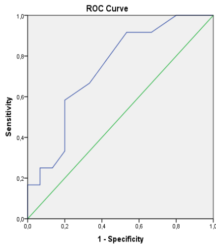
Figure 3. Receiver operating characteristic (ROC) analysis of increasing Beck depression scores and lower percentile (<33%) FORT ratios of the unexplained infertile group (AUC:0.73; 95% CI: 0.55-0.92; P=0.036).
