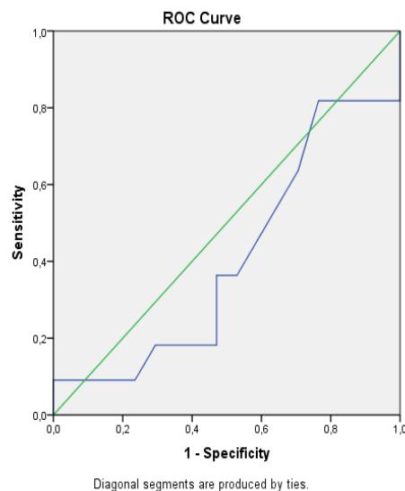
Figure 2. Receiver operating characteristic (ROC) analysis of increasing Beck depression scores and lower percentile (<33%) FORT ratios of the male factor group (AUC:0.40; 95% CI: 0.18-0.62; P=0.41).
